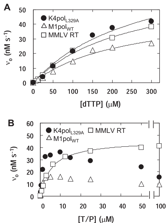
Fig. 3. Substrate dependence of the reaction rates ( v_0 ) in the reverse transcriptase reaction. The reaction was carried out with K4pol L329A (50 nM at 50 °C), M1pol WT (50 nM at 50 °C) or MMLV RT (2 nM at 37 °C). Solid line represents the best fit of the Michaelis–Menten equation. (A) Dependence of v_0 on the dTTP concentration. The initial T/P concentration was 10 μM. (B) Dependence of v_0 on the T/P concentration. The initial concentration of dTTP was 200 μM.
