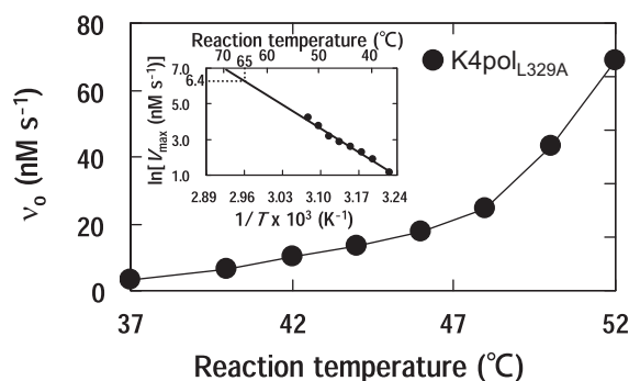
Fig. 4. Temperature dependence of the reaction rate ( v_0 ) of K4pol L329A in the reverse transcriptase reaction. The reaction was carried out with 50 nM K4pol L329A . The initial concentrations of dTTP and T/P were 200 and 25 μM, respectively. Inset shows Arrhenius plot.
