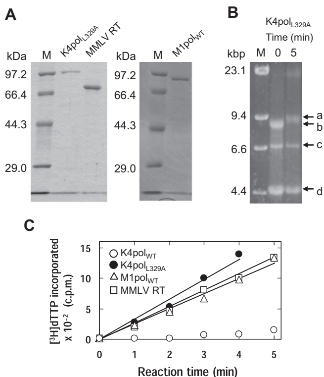
Fig. 2. DNA- and RNA-dependent DNA polymerase activities of K4pol L329A . (A) SDS-PAGE under reducing condition. Lane M, molecular-mass marker. (B) Agarose gel electrophoresis of reaction products in the DNA-dependent DNA polymerase assay. Lane M, molecular-mass marker. The DNA bands a, b, c, and d correspond to the gap-filled DNA, the gapped DNA (the annealing product of the 6789-base single-strand DNA fragment and the 7196-base single-strand circular DNA), the 6789-bp double-strand DNA fragment, and the 7196-base single-strand circular DNA, respectively. The reaction was carried out with 670 nM K4pol L329A at 50 °C for 5 min. (C) Incorporation of radioactivity of reaction products in the reverse transcriptase assay. The reaction was carried out with K4pol WT (50 nM at 50 °C), K4pol L329A (50 nM at 50 °C), M1pol WT (50 nM at 50 °C) or MMLV RT (2 nM at 37 °C). The initial concentrations of dTTP and T/P were 200 and 10 μM, respectively.
