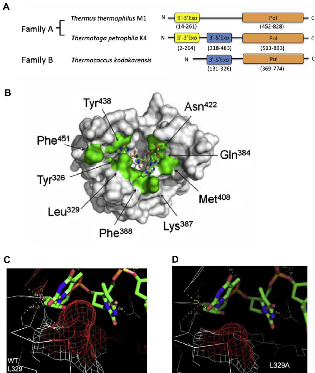
Fig. 1. Creation of reverse transcriptase activity in K4pol by the mutation of Leu329 → Ala. (A) Domain structure of bacterial DNA polymerases. (B–D) Modeled structure of K4pol-template RNA complex. The structure is constructed by Swiss model using E. coli Klenow fragment (1kfs) as a template. Carbon, nitrogen, oxygen, and phosphorus atoms of RNA are shown in green, blue, red, and orange, respectively. (B) Whole structure of K4pol WT -template RNA complex. The amino acid residues predicted to be located around an RNA template (Tyr326, Leu329, Gln384, Lys387, Phe388, Met408, Asn422, Tyr438, and Phe451) are shown in green. (C) Close-up view of Leu329 of K4pol WT -template RNA complex. (D) Close-up view of Ala329 of K4pol L329A -template RNA complex. Electron densities of the side chain of Leu329 (C) and Ala329 (D) are shown in red.
